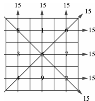
3-degree magic square
